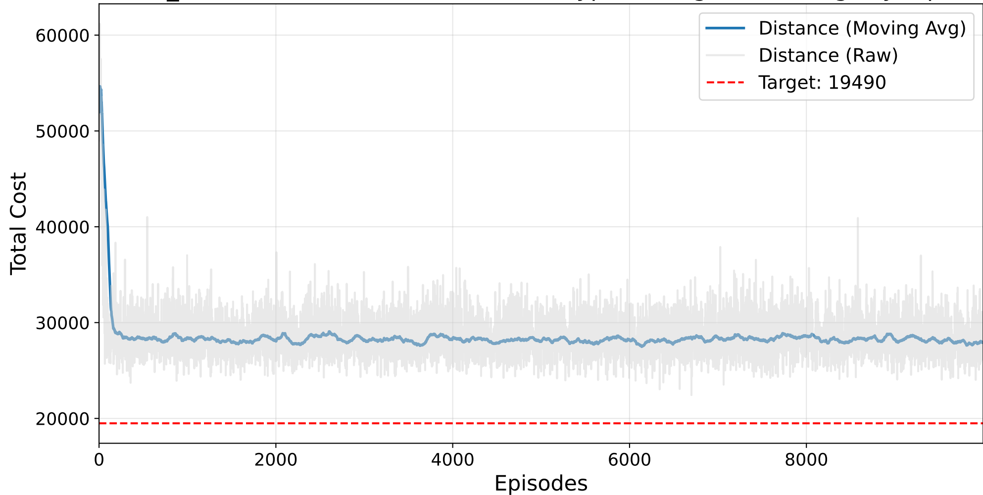
Final NO_BAYESIAN Masked AutoRL-SOP (HyperTuningSK) Training - ry48p.3.sop
